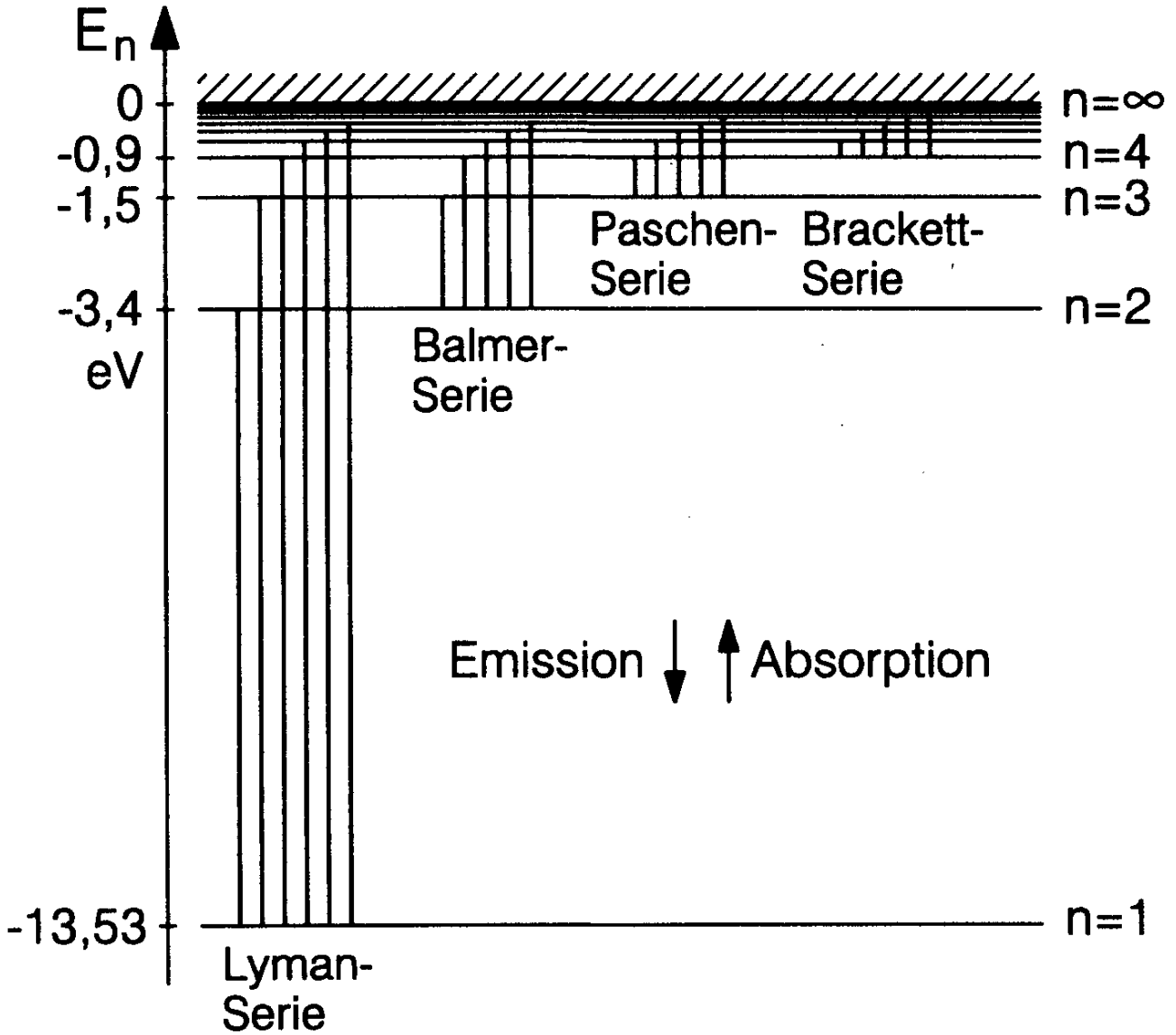
Figure 1: Energy level diagram for hydrogen showing the Lyman, Balmer, Paschen, and Brackett series.
